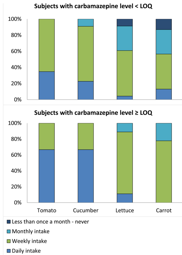
Figure 4. Association between baseline urinary carbamazepine levels and prestudy frequency of vegetable consumption in the entire study population ( N = 34 ). Top chart represents individuals with baseline levels < \text{LOQ} , bottom chart represents individuals with baseline levels \geq \text{LOQ} .
